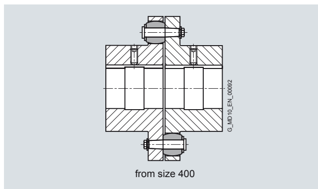
Types RWN/RWS – Alternate-sided arrangement of pins and buffers
