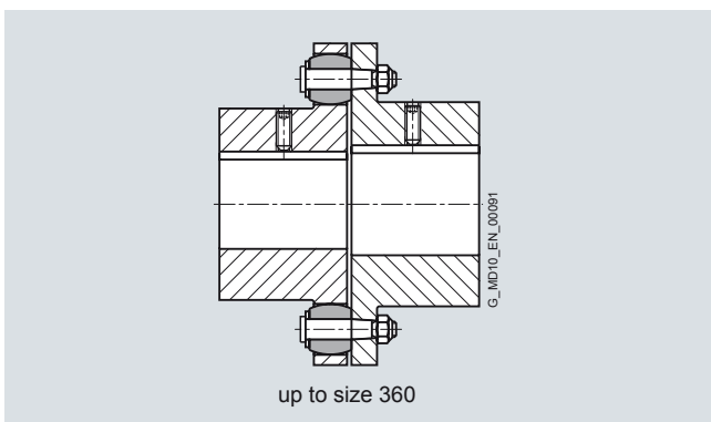
Types RWN/RWS – One-sided arrangement of pins and buffers
